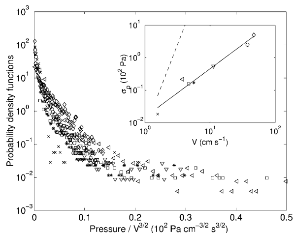
FIG. 3. Probability density functions of pressure fluctuations in the dilute cell rescaled by V^{3/2} ( V = 2\pi Af ), for different vibrational parameters as in Table I experiment No. 2 ( \times ); 3 ( \square ); 4 ( * ); 5 ( \triangleleft ); 6 ( \nabla ); 7 ( \circ ); 8 ( \diamond ). The inset displays the standard deviation \sigma_p \equiv \sqrt{\langle (p - \langle p \rangle)^2 \rangle} of pressure fluctuations p versus V . Power law fit of the form V^{3/2} (full line) and V^2 (dashed line).
