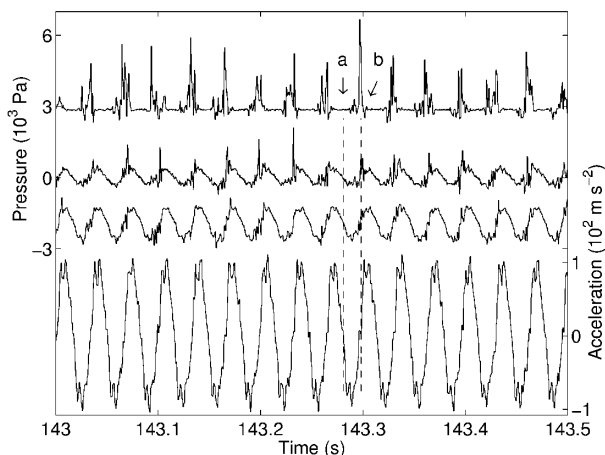
FIG. 2. From the lower to the upper curve: Time recordings of the acceleration in the direction of vibration, of the pressures in the densest cell, in the intermediate one, and in the dilute one. Letters a and b refer to the times when pictures in Figs. 1(a) and 1(b) have been taken. The parameters of vibration are the ones of experiment No. 8 in Table I. Pressure curves are shifted vertically for clarity.
